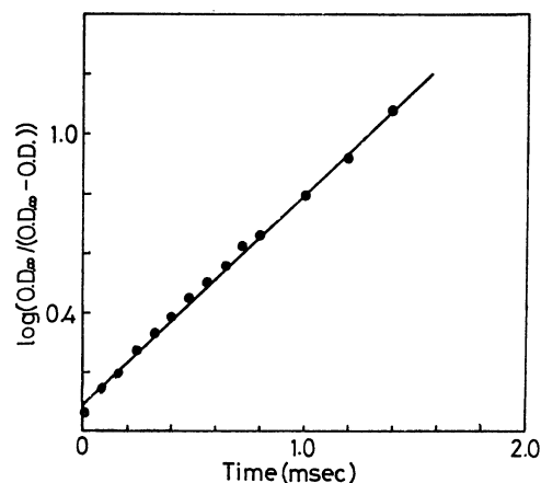
Fig. 4. First-order plot of appearance of the absorption at 340 nm observed by pulse radiolysis. ( 8 \times 10^{-4} M \text{NAD}^+ )
