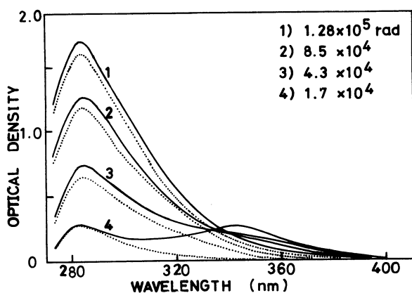
Fig. 1. The differential spectra of irradiated \text{NAD}^+ solutions ( 2 \times 10^{-4}\text{M} ) immediately after irradiation (solid line) and two days after irradiation (dotted line). Dose rate was 2.8 \times 10^4 \text{ rad} \cdot \text{hr}^{-1} .
