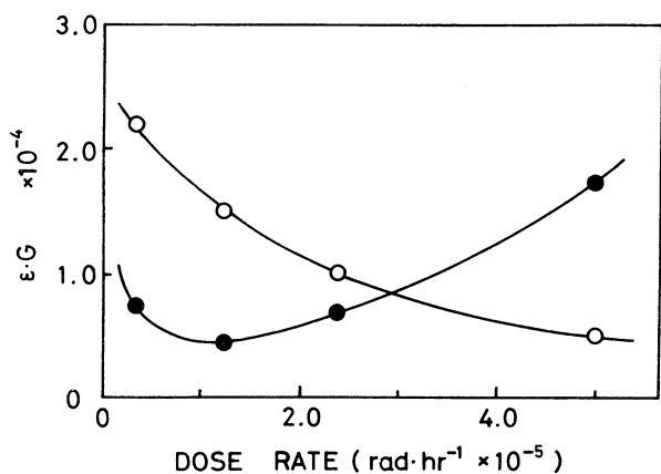
Fig. 3. The \epsilon \cdot G values at 283 nm (closed circles) and 340 nm (open circles) against dose rate. (Total dose: 3 \times 10^4 rad, 1.5 \times 10^{-4} M \text{NAD}^+ )
