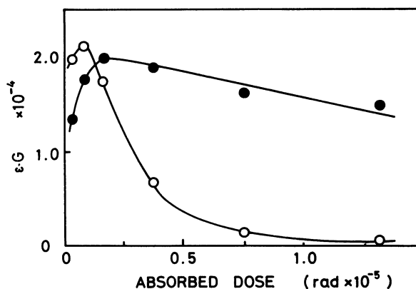
Fig. 2. The \epsilon \cdot G values of irradiated \text{NAD}^+ solution ( 2 \times 10^{-4}\text{M} ). Dose rate was 2.8 \times 10^4 \text{ rad} \cdot \text{hr}^{-1} . Observed at 283 nm (closed circles) and 340 nm (open circles).
